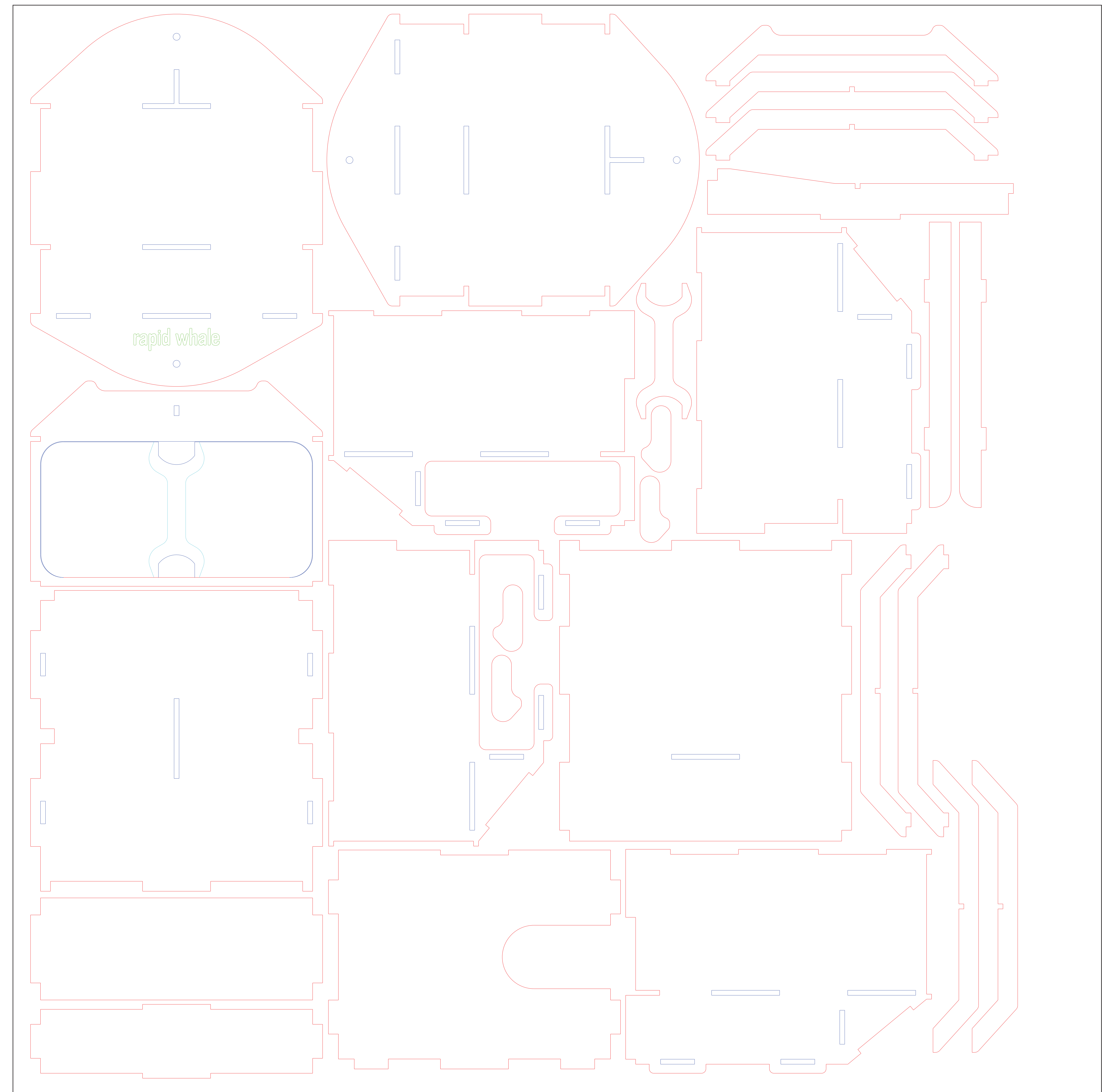
SHEET REF NAME: WOOD BODY + Extra Bits MATERIAL: 1/8" (actual: ~0.110") Mahogany Wood Sheet SIZE: 24"x24" SPECIAL INSTRUCTIONS: Pretty side UP
