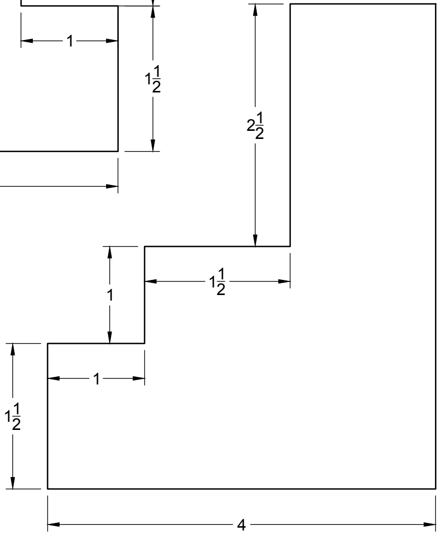
Post Supports (all dimension in inches)
